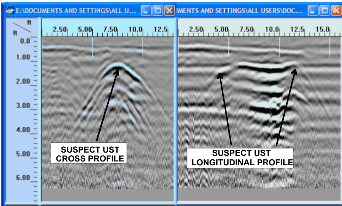
Typical Ground-penetrating radar cross and longitudinal profiles completed over a single UST-like feature.
