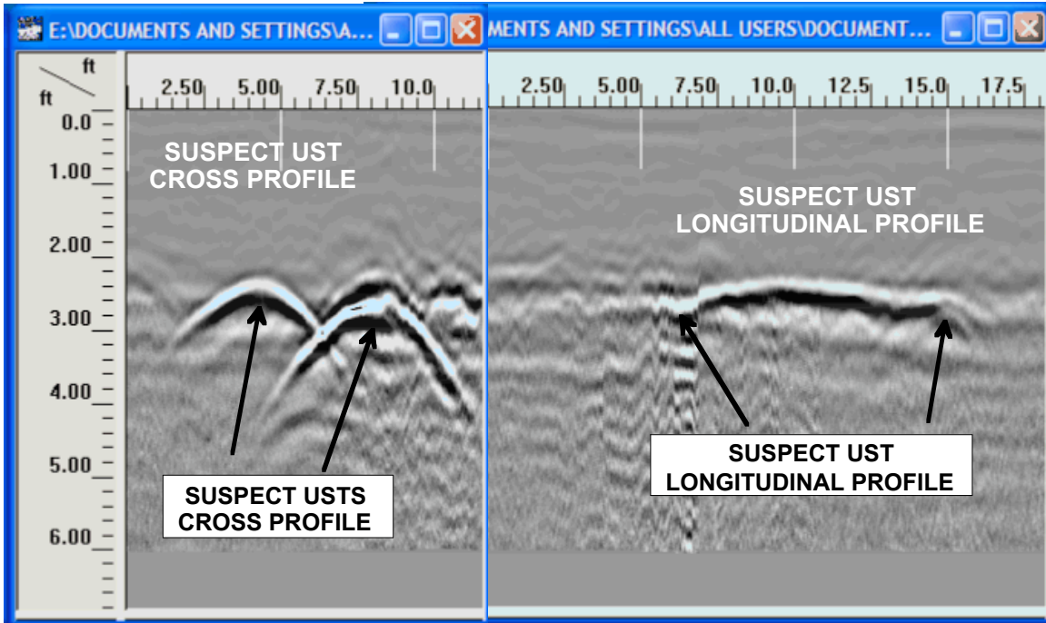
Typical Ground-penetrating radar cross and longitudinal profiles completed over two UST-like features.
